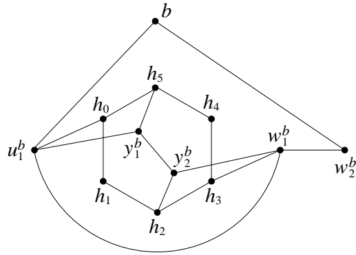
Figure 2: The subgraph of G' added around a vertex b \in G_B \setminus S_B , together with the 6-cycle S .
