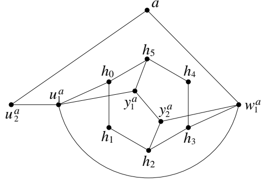
Figure 1: The subgraph of G' added around a vertex a \in G_A \setminus S_A , together with the 6-cycle S .
