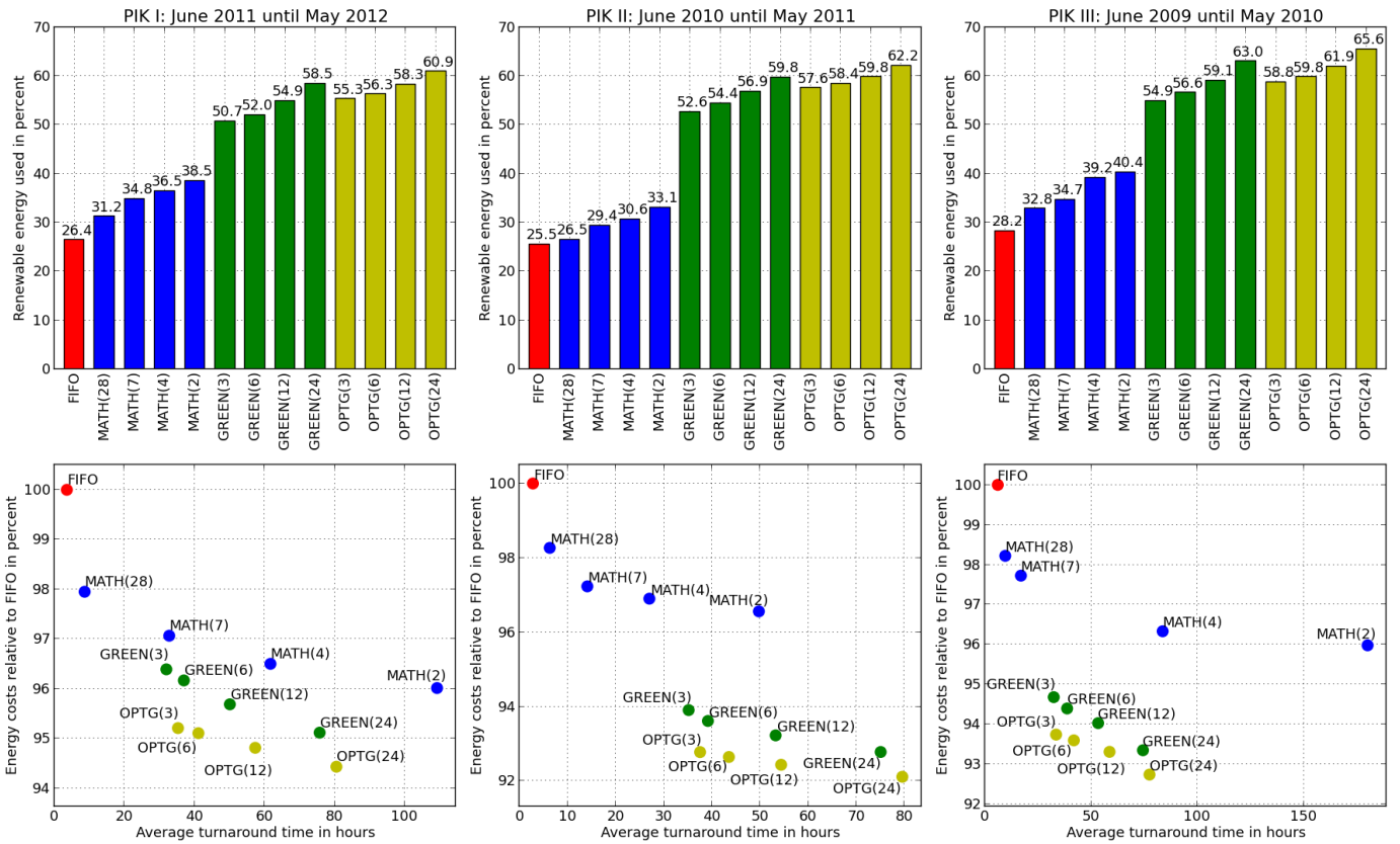
Fig. 4: Comparison of the PIK simulation results with different configurations
