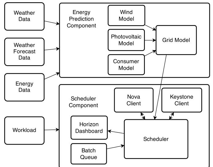
Fig. 2: Green Control Centre architecture diagram
